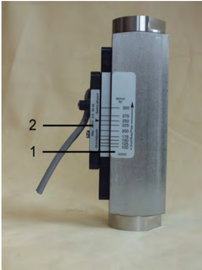
Fig. 1: Flow monitor RVM/U-L1
