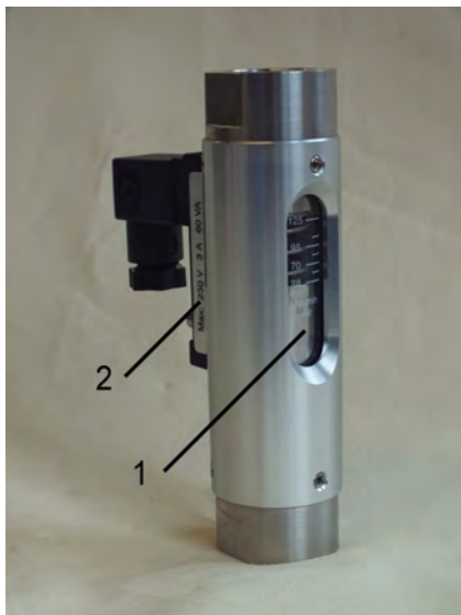
Fig. 1: RVO/U-L2 flow monitor
