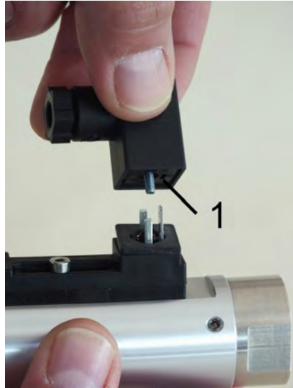
Fig. 53: Remove the female socket
