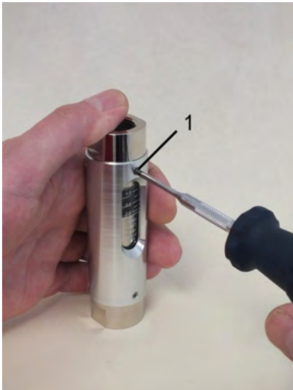
Fig. 35: Remove the process connection (outlet)
