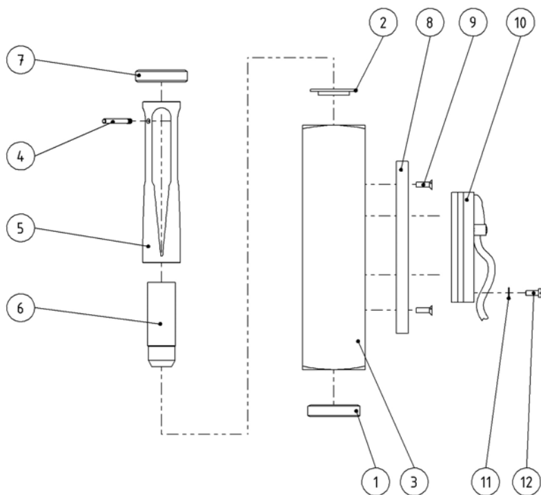
Fig. 7: Type DWM-L50 through DWM-L100 (G1")
