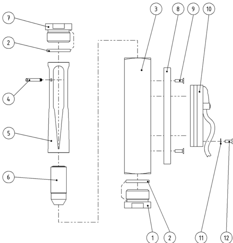
Fig. 5: Type DWM-L1,5 through DWM-L18
