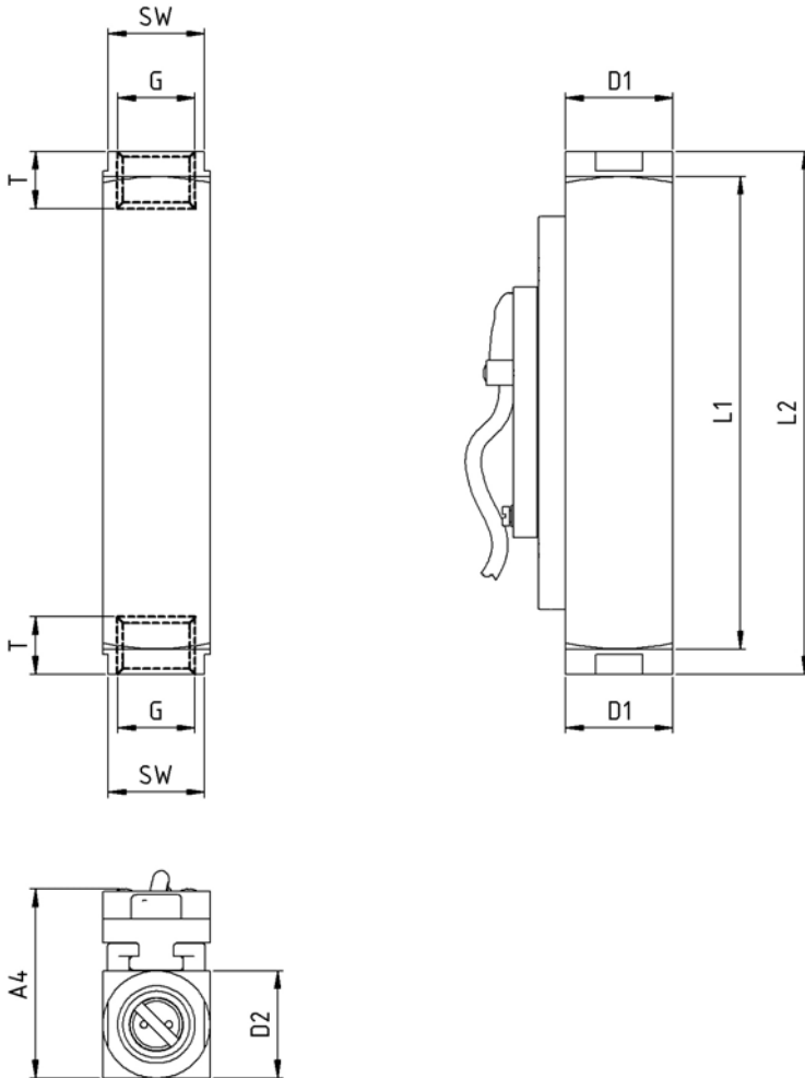
Fig. 2: Type DWM-L1,5 through DWM-L18
