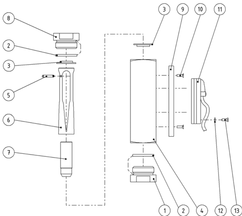
Fig. 6: Type DWM-L18 through DWM-L50 (G3/4")
