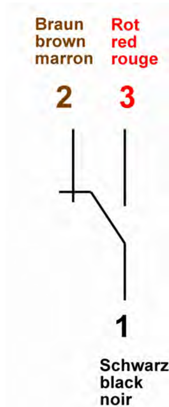
Fig. 20: Switch position under no-flow condition
