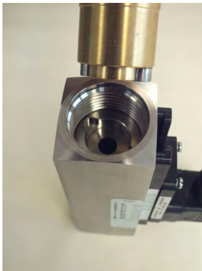
Fig. 37: Insert threaded ring insertion tool (outlet)
