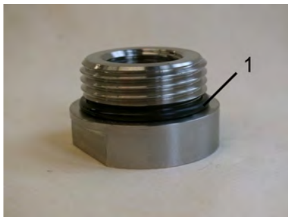
Fig. 48: Properly positioned O-ring
